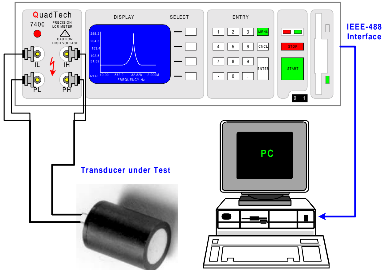
Figure 1: Connection of Transducer to 7400 Precision LCR Meter
